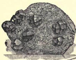
Garnet crystals in mica schist.
